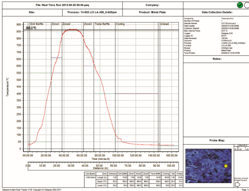
Figure 5-16 860 °C Thick Film profile
