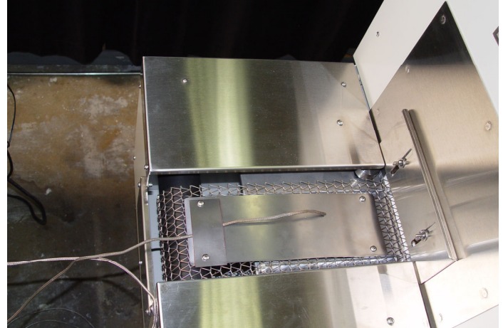
Figure 5-8 Metal Plate Sample with Wire Sheath Type K Thermocouple
