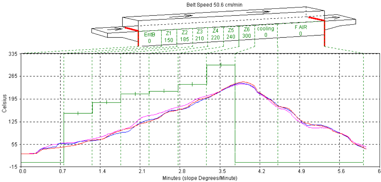
Figure 5-2 Temperature Profile
