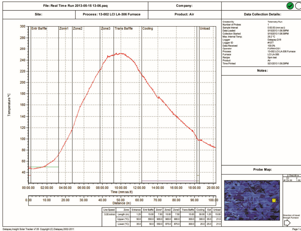
Figure 5-15 250 °C Curing Profile
